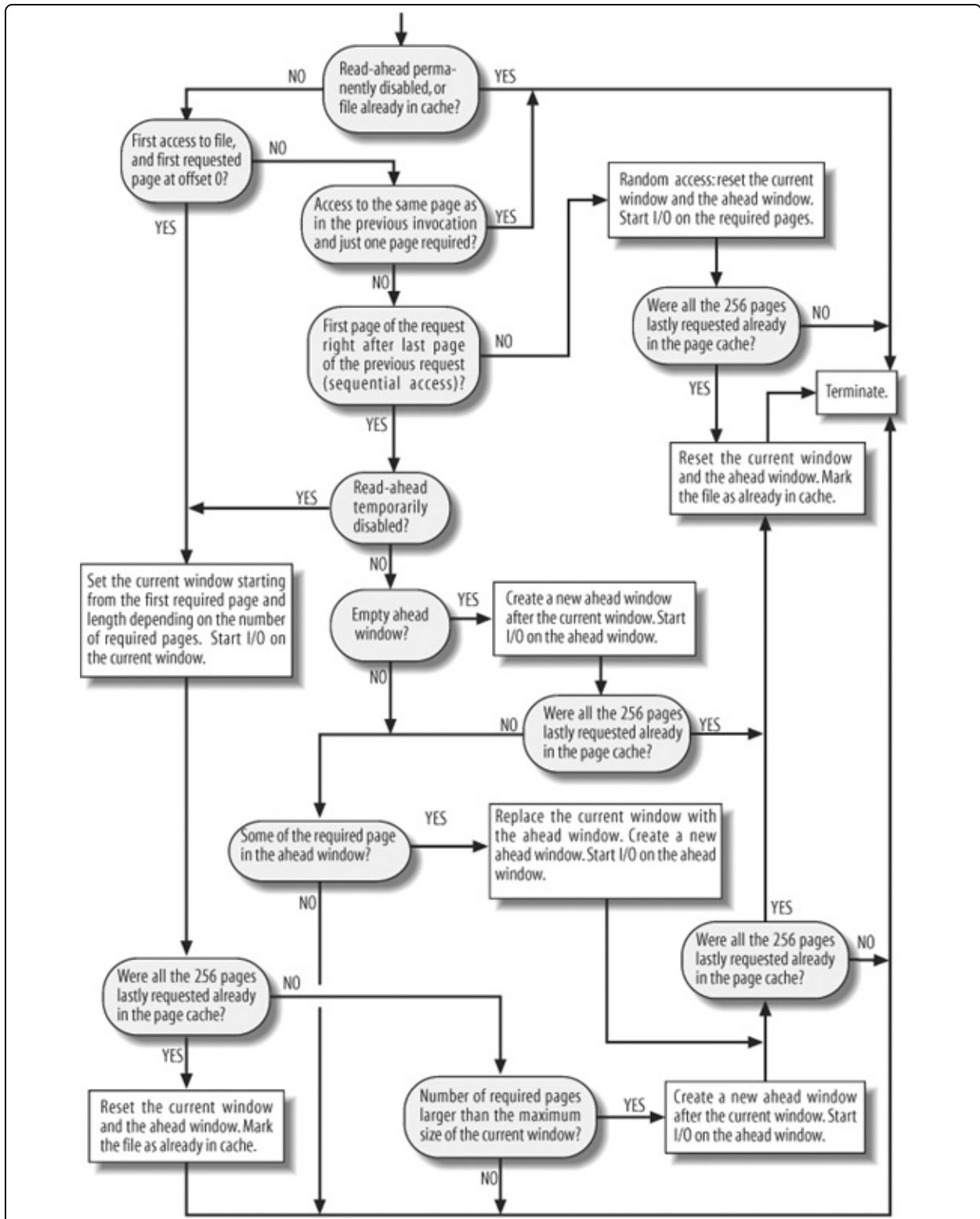
Figure 16-1. The flow diagram of the page_cache_readahead( ) function
